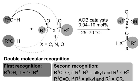
Scheme 1. Representative scheme of alcoholysis of 1 catalyzed by AOBs. The basis of the selectivity of the recognition by the AOB of the alcohol (first recognition) and of the dicarbonyl unit (second recognition) is shown. R^1 and R^2 differ in steric size, electronic nature, and functional groups. Dashed arrows denote relatively unfavorable nucleophilic attack.
