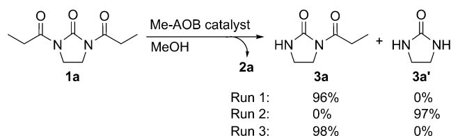
Scheme 2. Methanolysis of 1a . Product 2a is methyl propionate. Run 1: Me-AOB (1 mol %), 25 °C, < 15 min; Run 2: Me-AOB (2 mol %), 50 °C, 15 h; Run 3: Me-AOB (0.04 mol %), 25 °C, 21 h.
